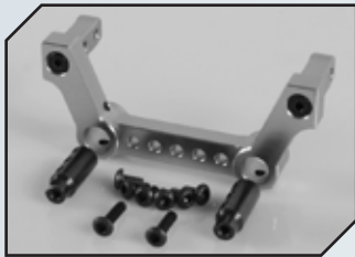
Art.Nr.: RC4ZS1002 RC4WD Blade Snow Plow Mounting kit
